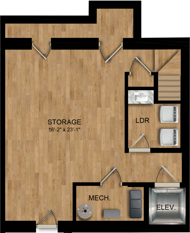
Cellar Plan
